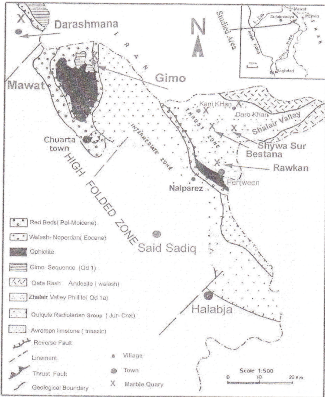
Fig.(1) Geological map of Mawat and Penjween Area (Jassim and Al-Hassan, 1977[4]). The map is Used for showing location of Marble quarries.
